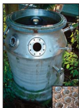
STOCK CODE: N7520-19 38 SQ.M. S/S CHEMTEC EVAPORATOR COLUMN
