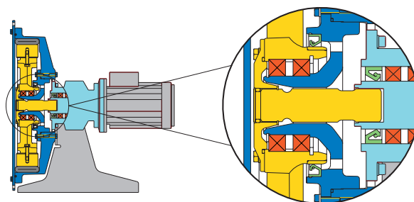
Bredel direct-coupled
