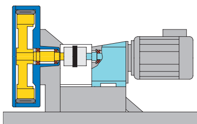
Long-coupled
